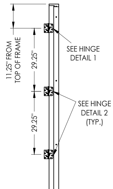
6'8 HINGE JAMB/MULLION
