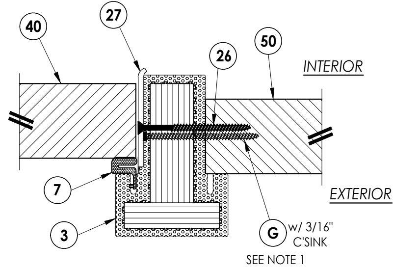
3 3 HORIZONTAL CROSS SECTION Shown Direct to masonry Inswing
