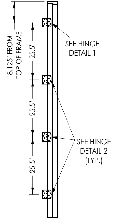
8'0 HINGE JAMB/MULLION
