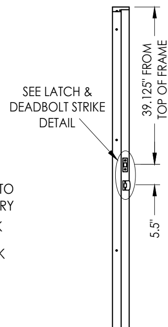
6'8 STRIKE JAMB/MULLION
