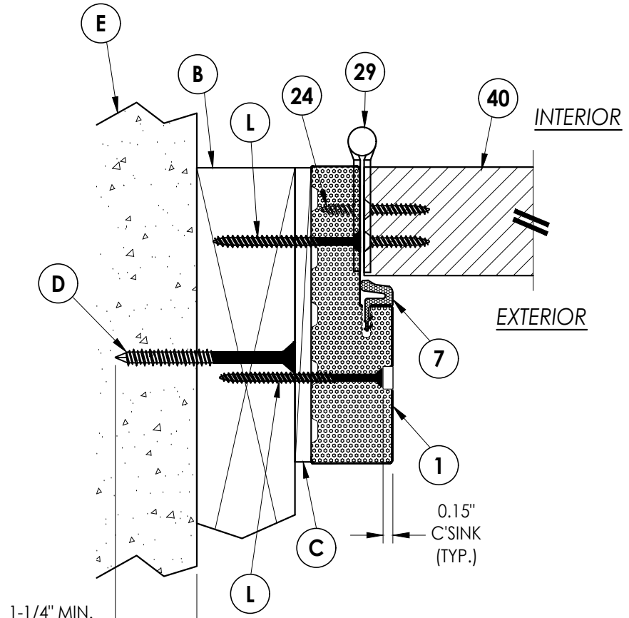
4 3 HORIZONTAL CROSS SECTION Shown with 2X Buck Inswing
